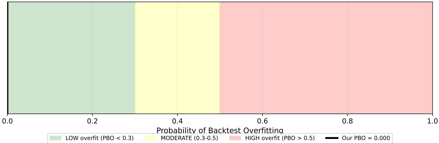
Figure 4: Probability of Backtest Overfitting (PBO) Bailey/Borwein/López de Prado/Zhu 2014 — ? strategies, ? obs
