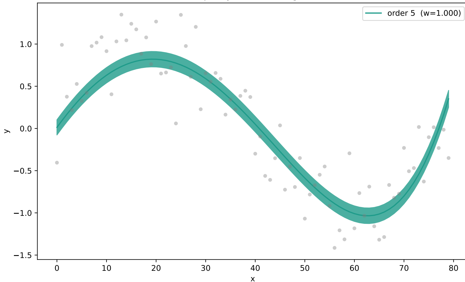
Per-model predictive distributions (opacity \propto model weight)
