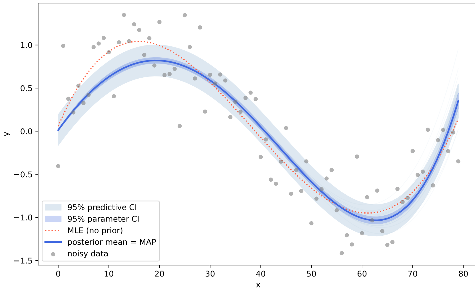
Polynomial Fitting 5th Order: Bayesian Approach (zero-mean Gaussian prior)
