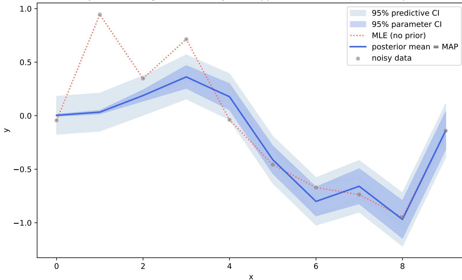
Polynomial Fitting 9th Order: Bayesian Approach (zero-mean Gaussian prior)
