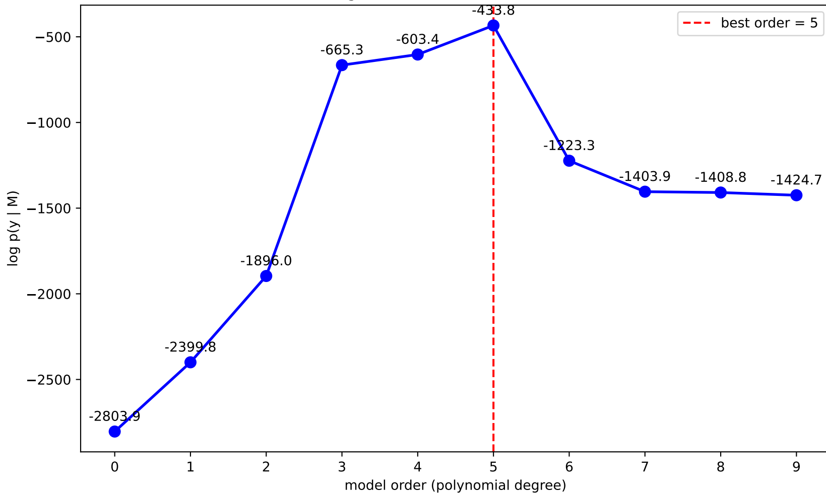
Marginal likelihood vs model order
