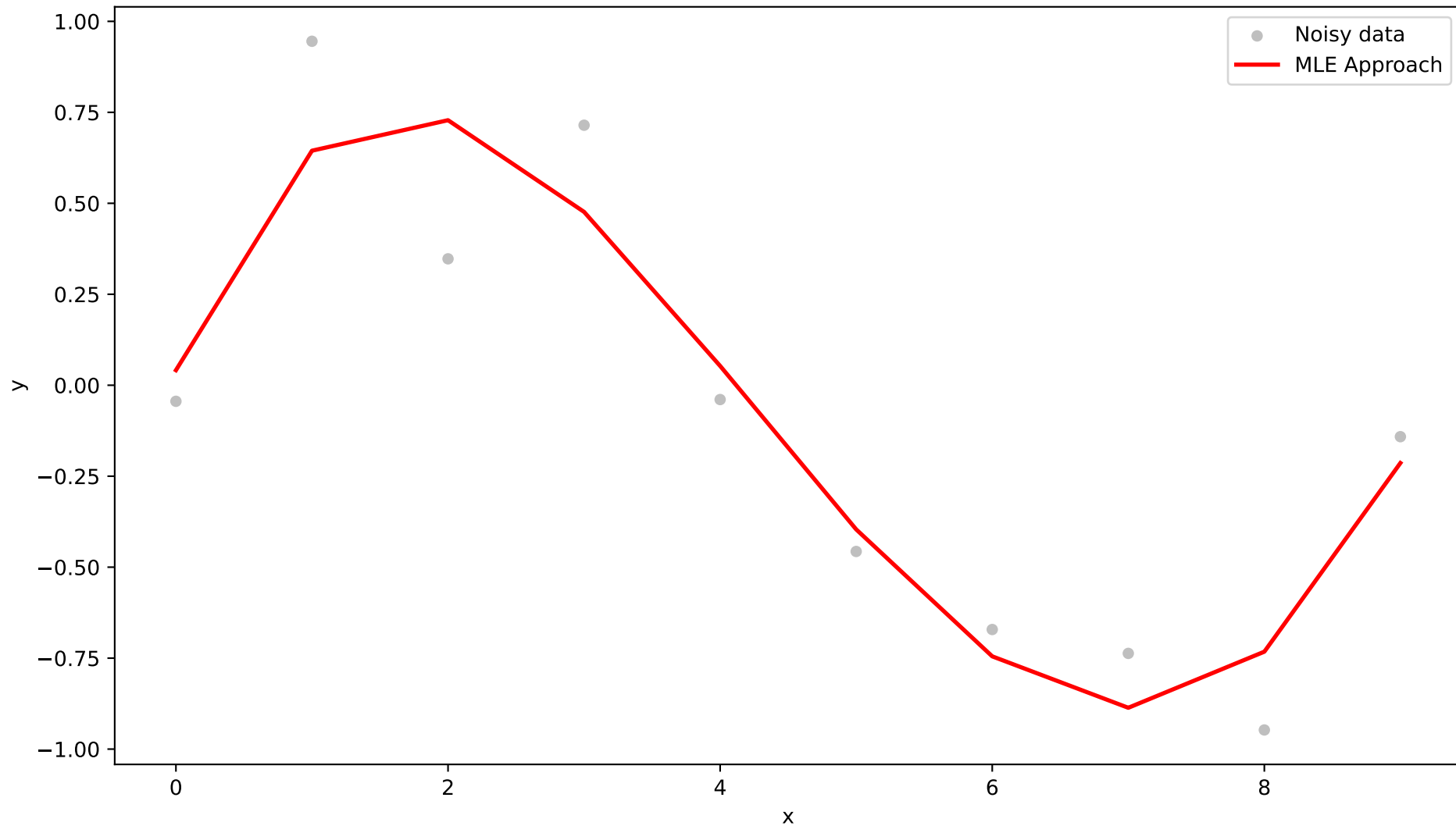
Polynomial Fitting 4th Order: MLE
