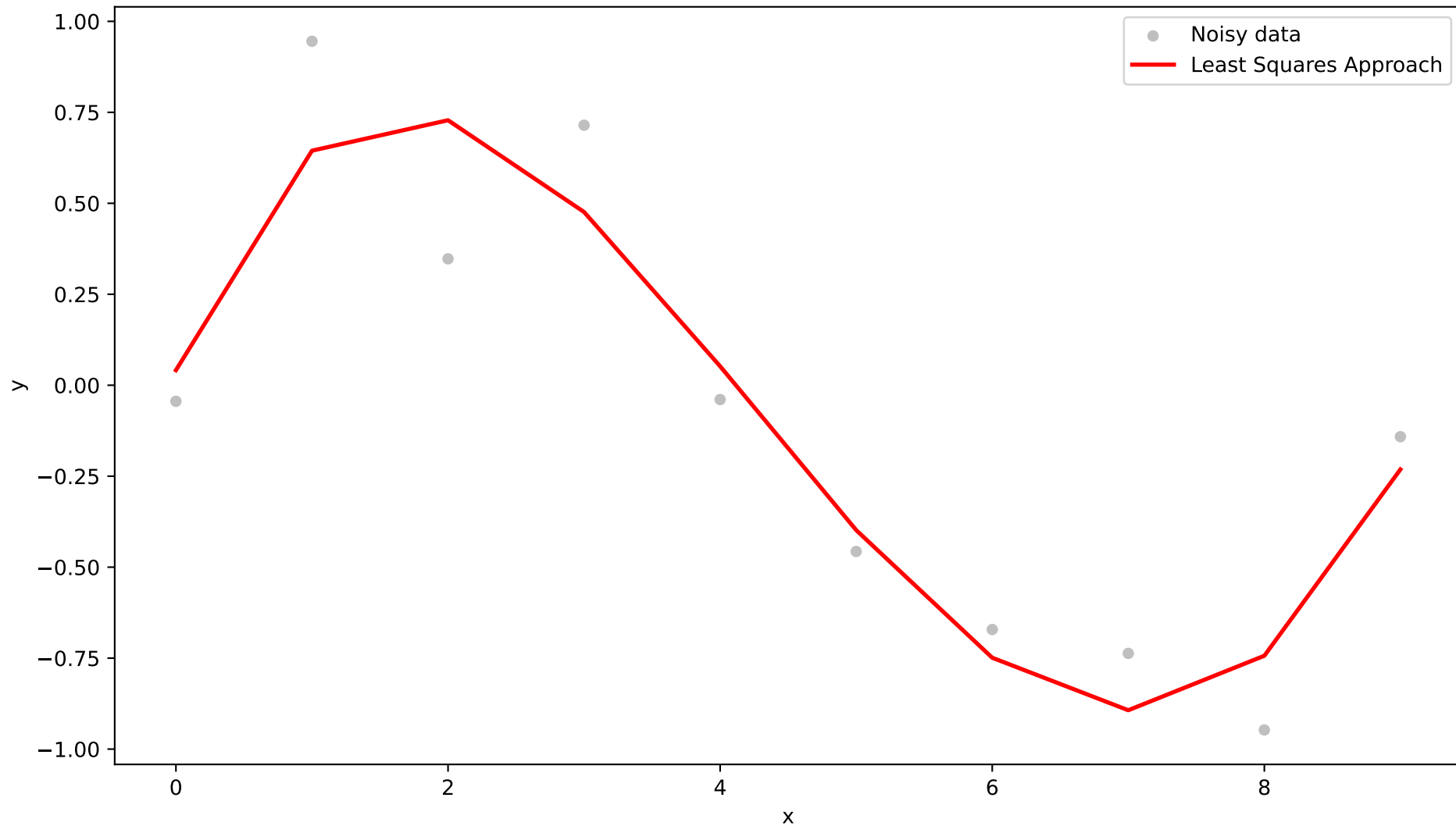
Polynomial Fitting 4th Order: Least Squares
