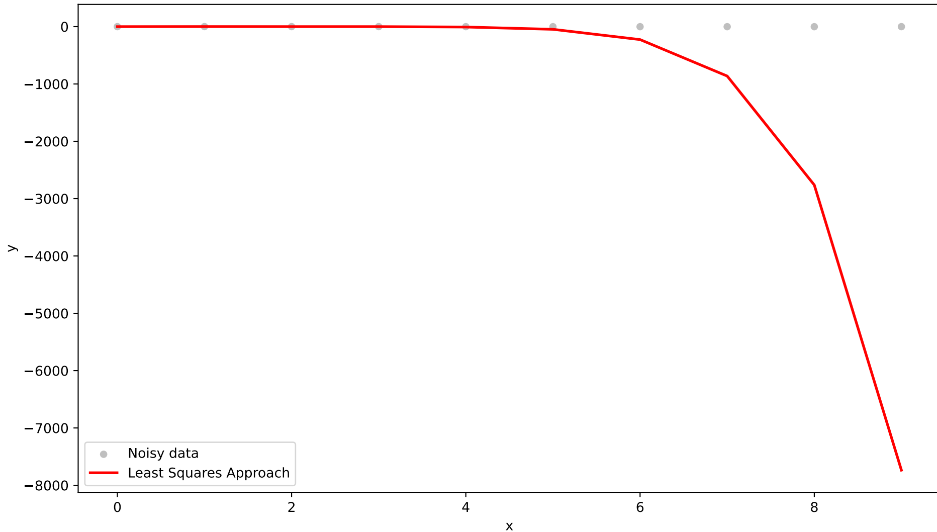
Polynomial Fitting 9th Order: Least Squares
