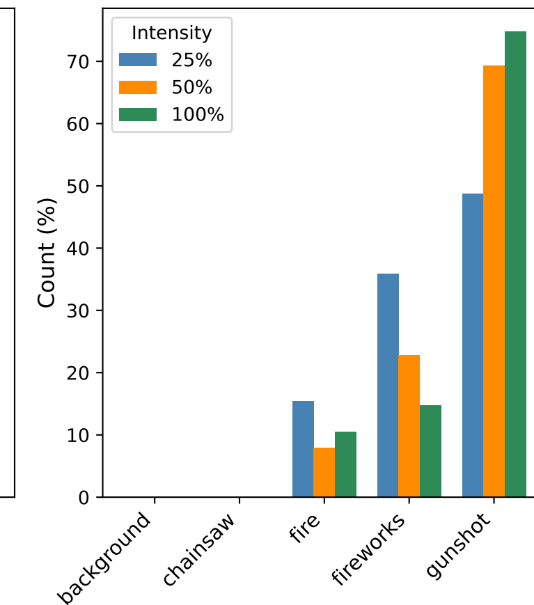
GUNSHOT - HF
