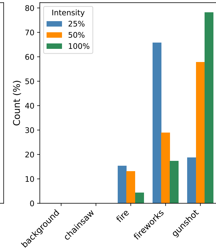
FIREWORKS - HF
