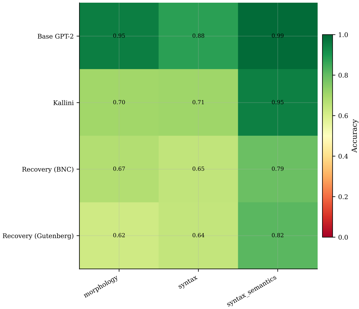
BLiMP Accuracy by Field | Hop
