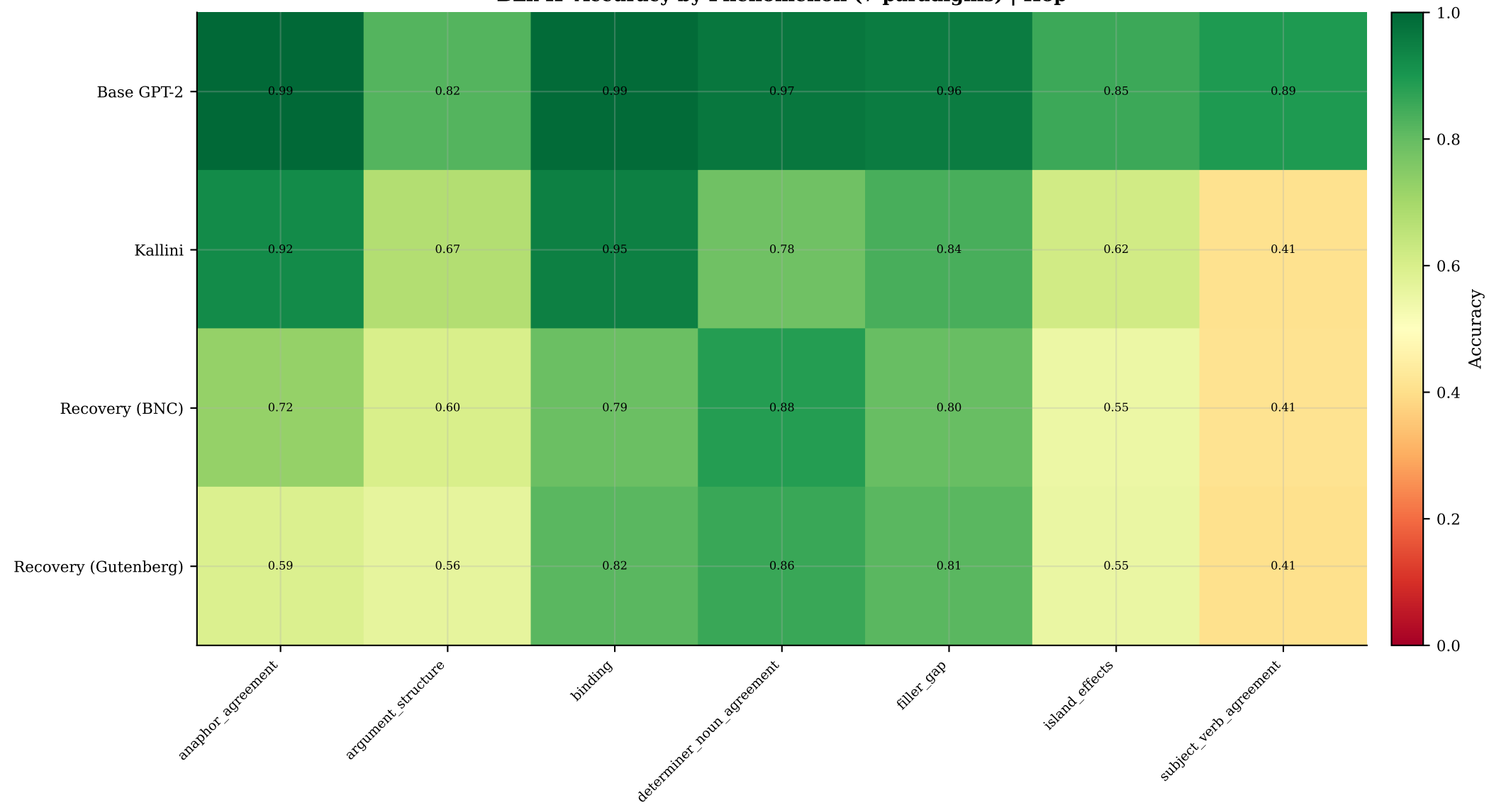
BLiMP Accuracy by Phenomenon (7 paradigms) | Hop
