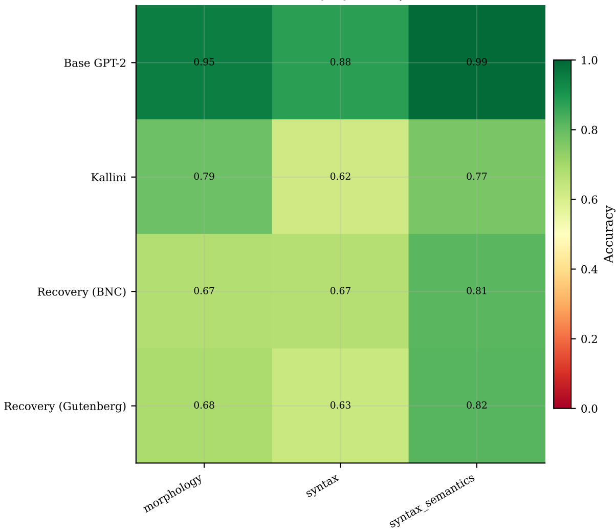
BLiMP Accuracy by Field | Local-W3
