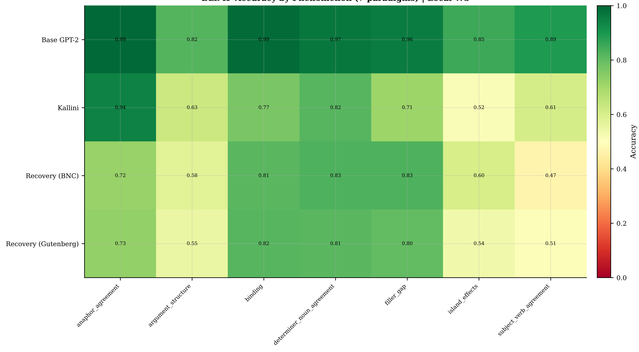
BLiMP Accuracy by Phenomenon (7 paradigms) | Local-W3
