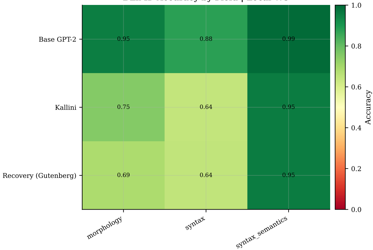
BLiMP Accuracy by Field | Local-W5
