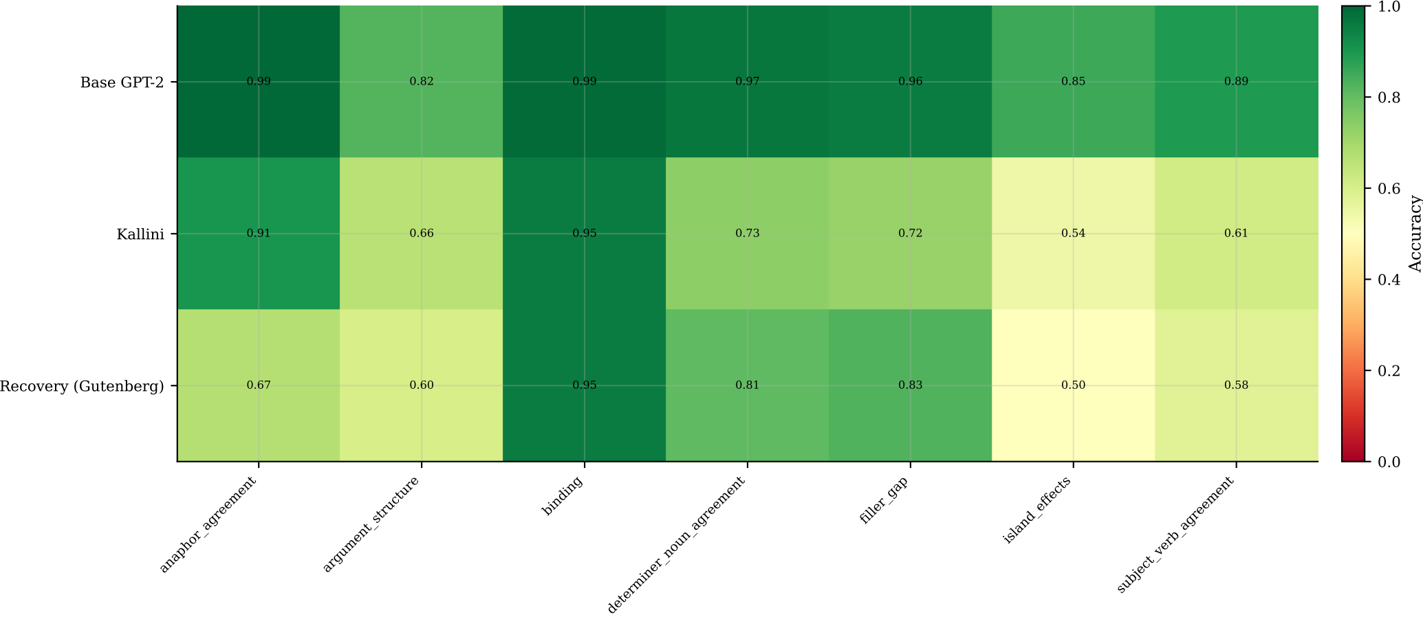
BLiMP Accuracy by Phenomenon (7 paradigms) | Local-W5
