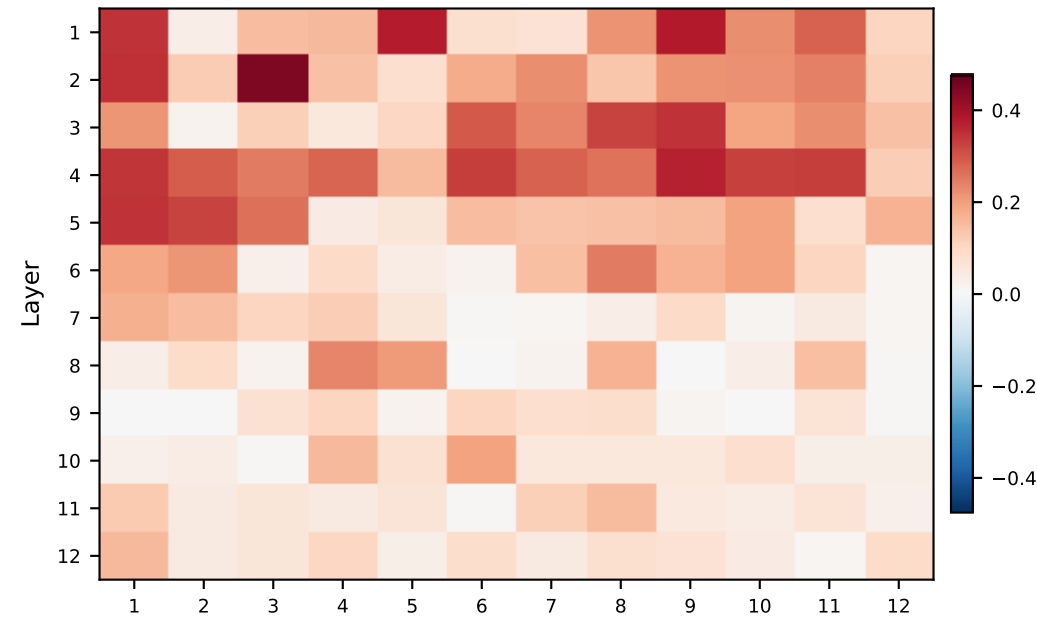
Recovery (Guten)
