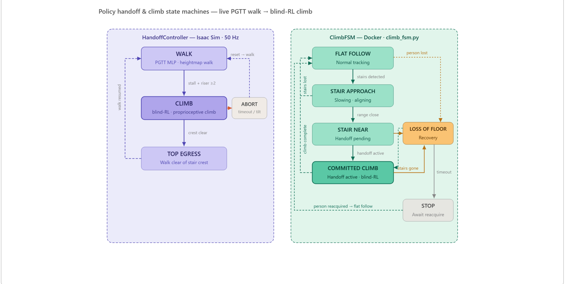
Fig. 8 — HandoffController (Isaac Sim, 50 Hz) and ClimbFSM (Docker) run concurrently via UDP.
