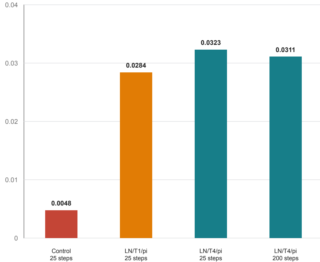
Mean quantum-weight gradient norm
