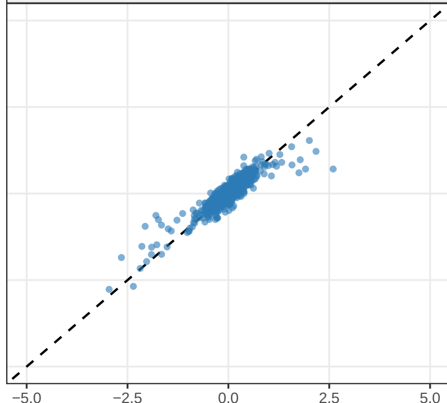
ROBU Algorithm
