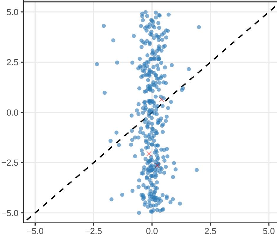
Standard MM-Estimator
