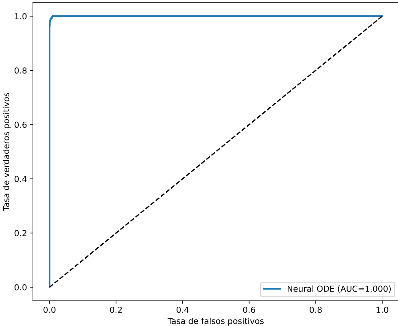
Curva ROC - Test
