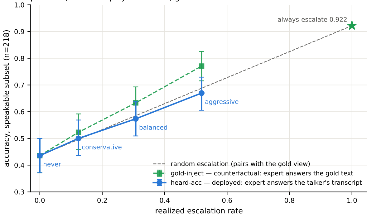
Accuracy vs escalation rate — speakable subset (“TTS-fair” view) probe v2; blue = deployed channel, green = channel-controlled counterfactual
