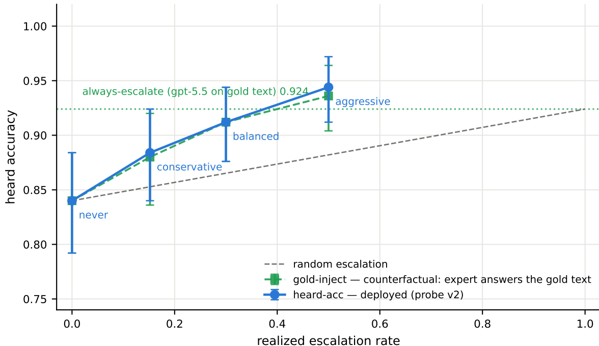
Accuracy vs escalation rate — Speech Llama Questions (OpenAudioBench, n=250) probe v2, per-domain quantile thresholds; scored with OpenAudioBench's own judge (gpt-4o)
