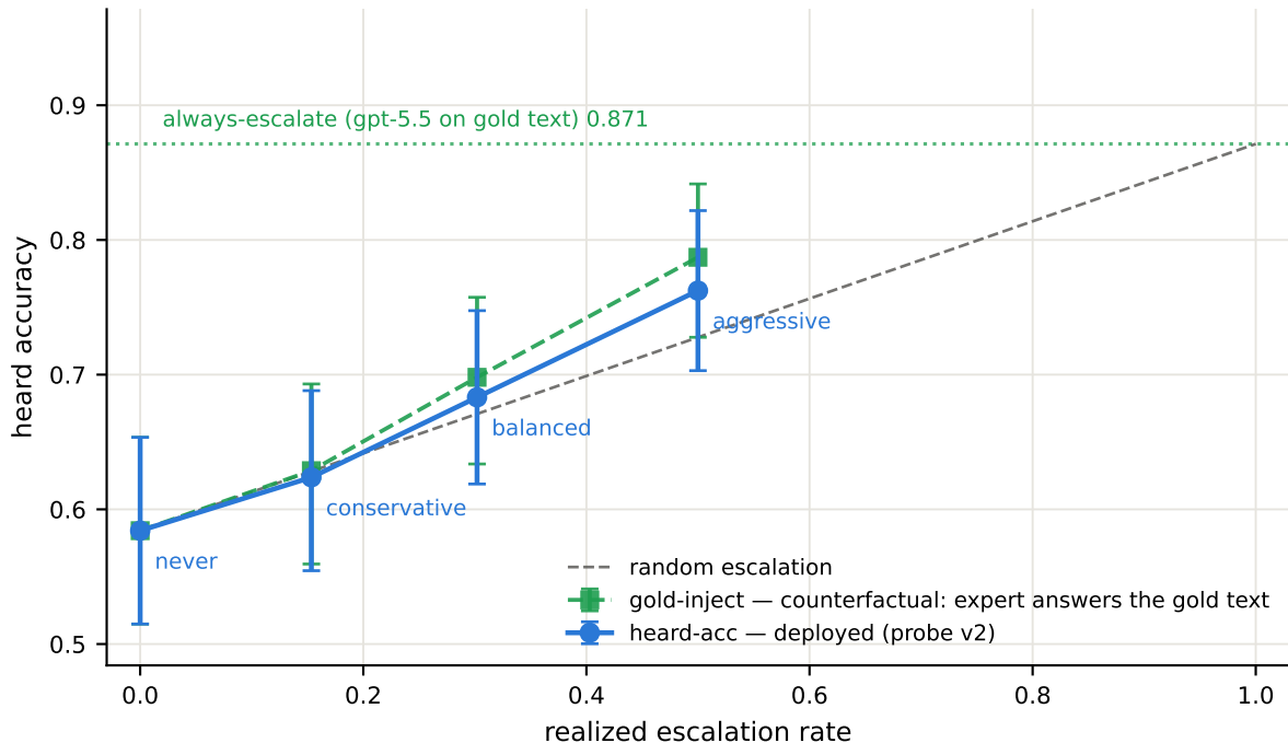
Accuracy vs escalation rate — Speech Reasoning QA — Chinese (OpenAudioBench, n=202) probe v2, per-domain quantile thresholds; our reference-anchored judge
