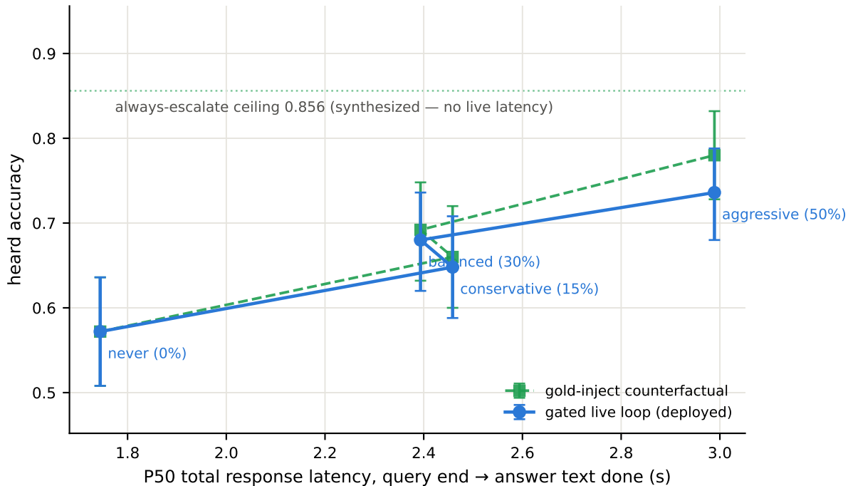
What latency buys — Speech Web Questions (OpenAudioBench, n=250) (points = escalation arms, labelled by escalation rate)
