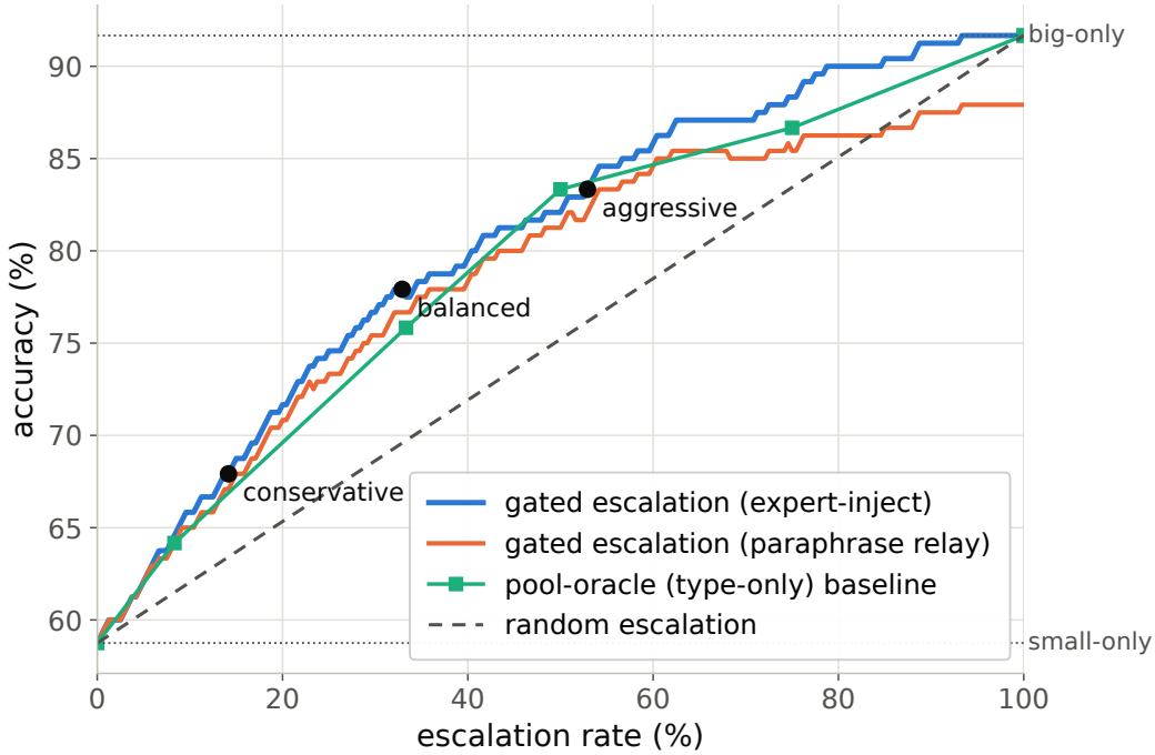
Figure 9: Accuracy vs. escalation rate, frozen test split: gated escalation vs. random-escalation and pool-oracle (type-only) baselines between the small-only and big-only endpoints.
