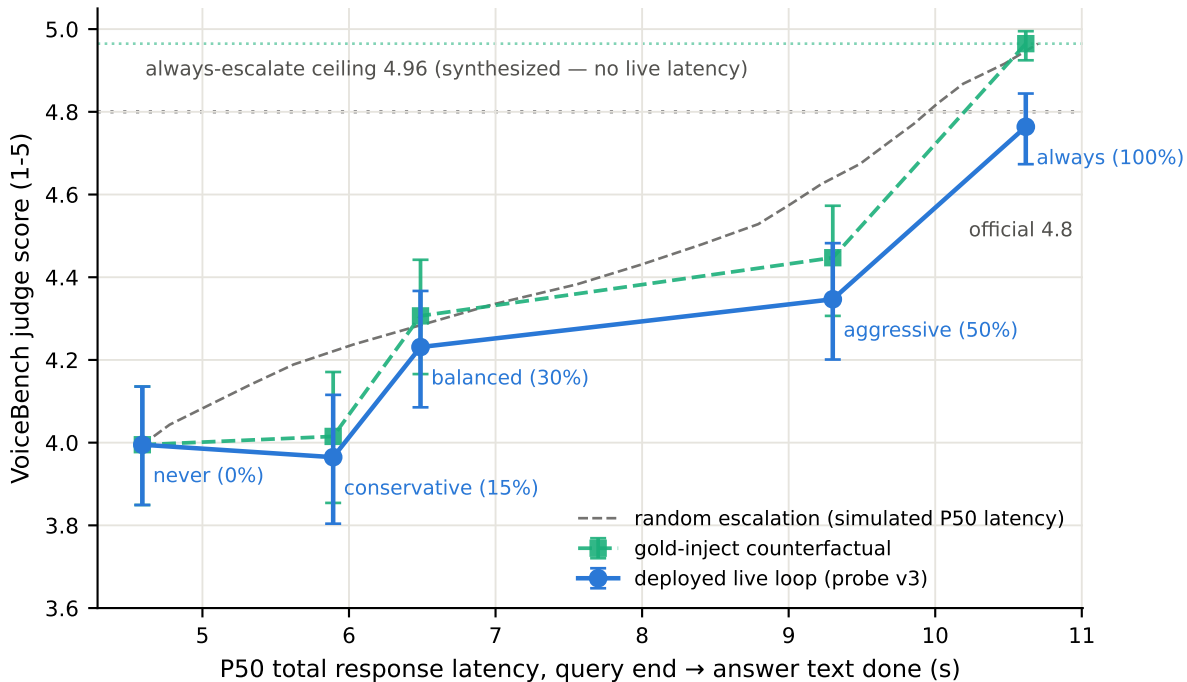
What latency buys — VoiceBench AlpacaEval (n=199) probe v3, per-domain quantile thresholds; VoiceBench's own gpt-4o-mini judge prompt (1-5)
