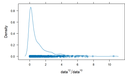
(b) Densityplot
