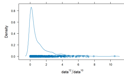
(b) Densityplot
