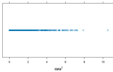
(c) Stripplot
