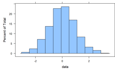
(a) Histogram
