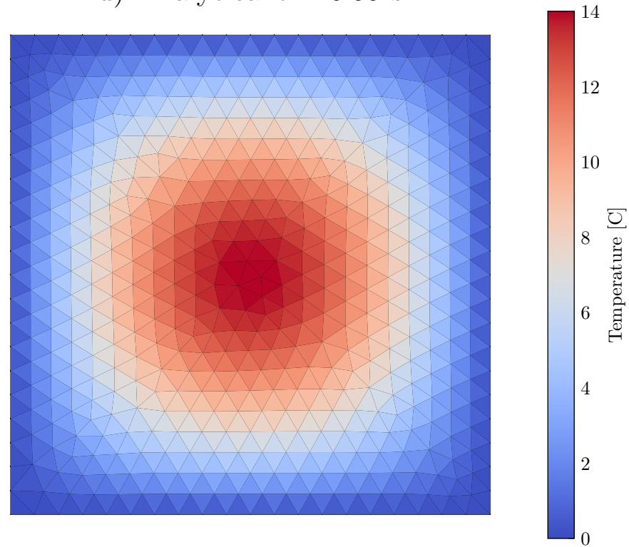
d) Analytical t = 0.99 s
