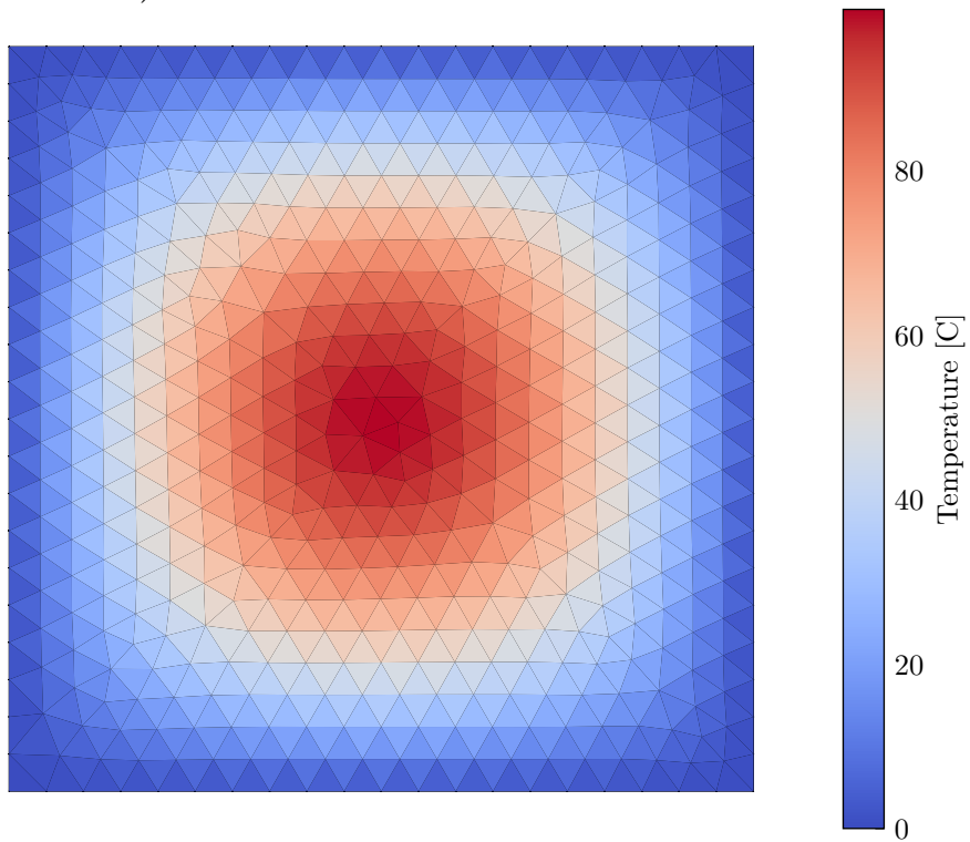
a) Initial condition t = 0 s
