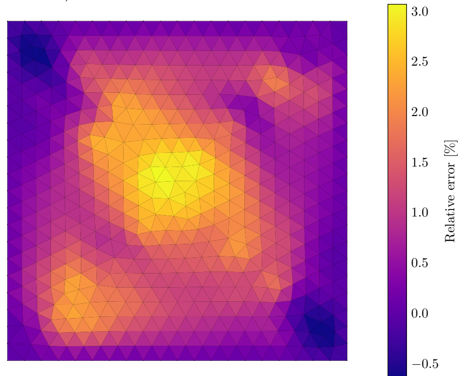
b) Relative error t = 0.99 s
