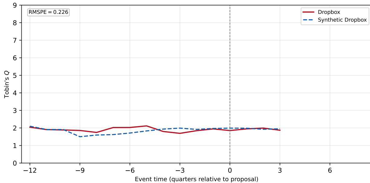
Covariate balance
