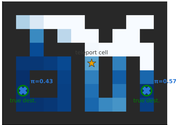
best-of-K (ours, router \pi )
