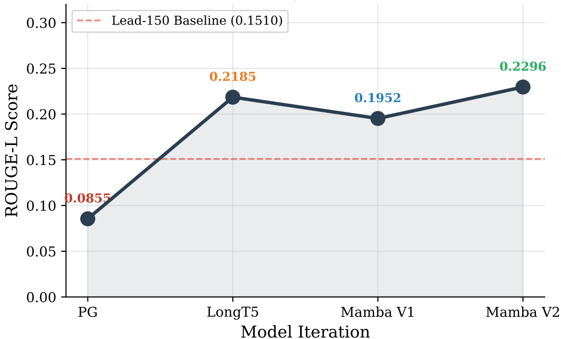
ROUGE-L Score Progression Across Models
