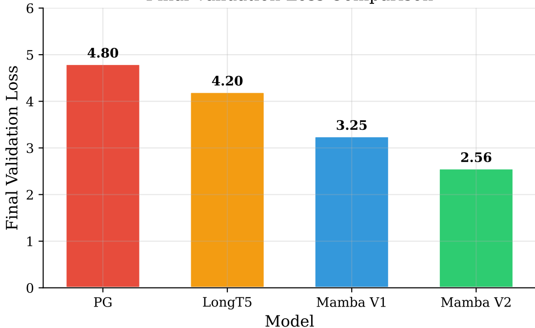
Final Validation Loss Comparison
