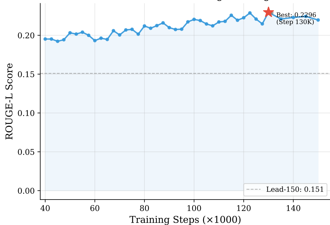
ROUGE-L Score During Training
