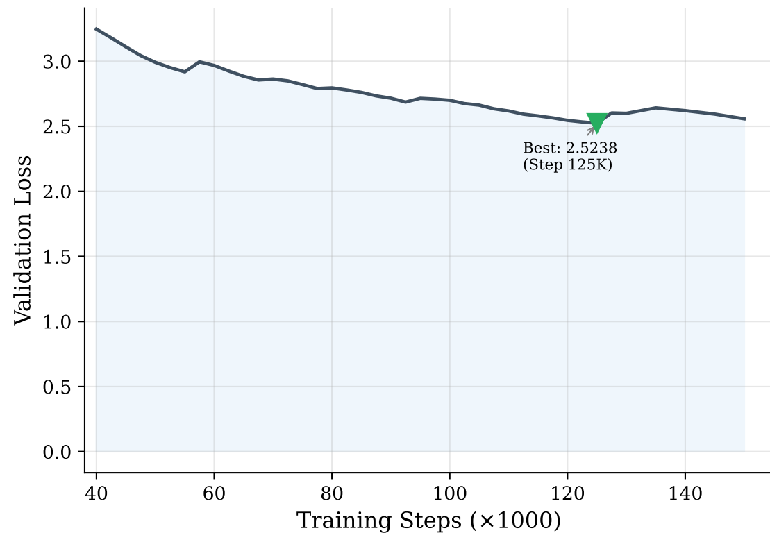
Validation Loss Curve
