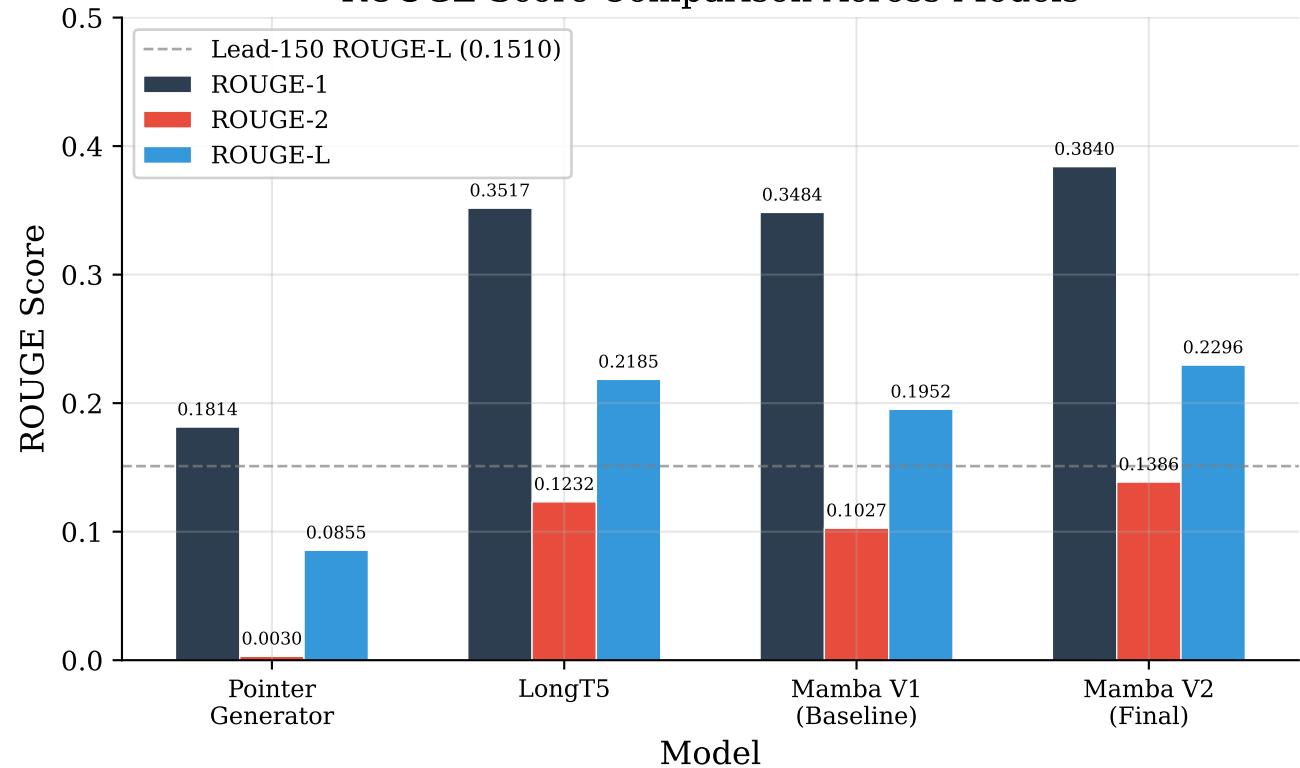
ROUGE Score Comparison Across Models
