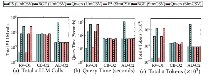
Figure 8: Comparisons of Using Different Embedding Models
