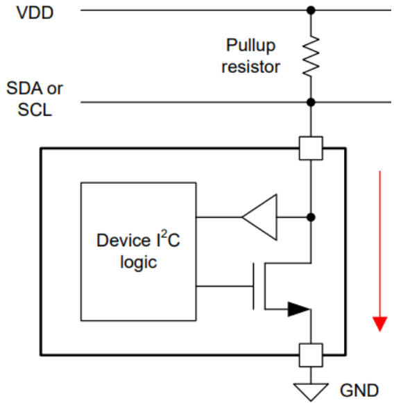
Figure 2.2: Open Drain.
