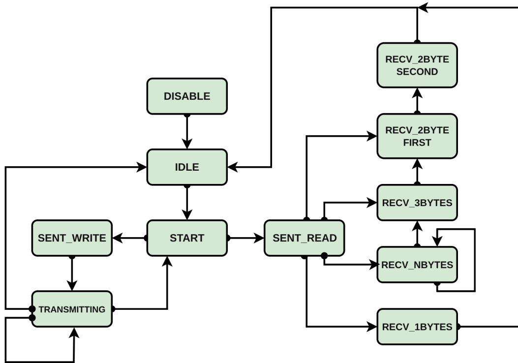
Figure 4.3: stm32f405 i2c controller fsm
