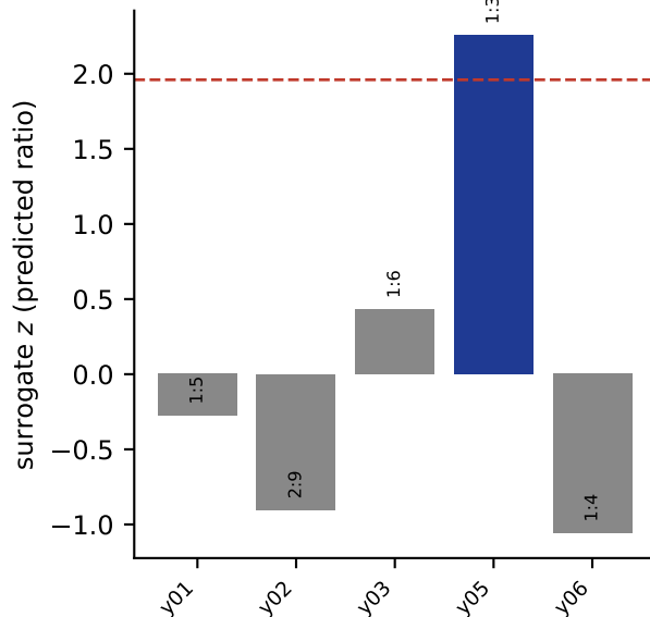
B 1/5 subjects locked ( p \leq 0.05 )
