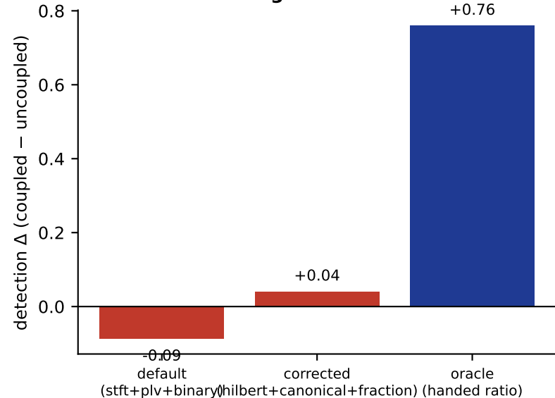
A Default config anti-detects a 2:3 lock
