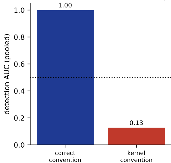
B The swapped-multiplier bug
