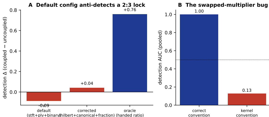
Figure 2: Default settings anti-detect a known lock. (A) Detection margin (coupled – uncoupled) for a clean 2:3 lock: the default configuration is negative (anti-detection), the corrected configuration recovers the sign, the oracle separates cleanly. (B) The swapped-multiplier convention alone drives detection below chance; the canonical convention restores it.
