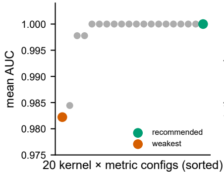
A Accuracy saturates (0.982–1.000) B Rotation number \rho(\Omega) → choose on speed (harmsim ~27× faster) (forced Van der Pol: 1:1 lock)
