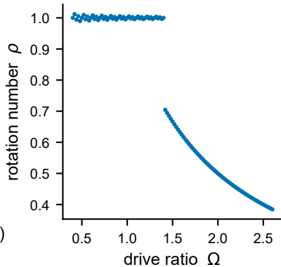
A Accuracy saturates (0.982–1.000) B Rotation number \rho(\Omega) → choose on speed (harmsim ~27× faster) (forced Van der Pol: 1:1 lock)
