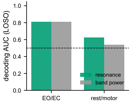
A EEG state decoding (LOSO AUC) (EO/EC \approx band power)
