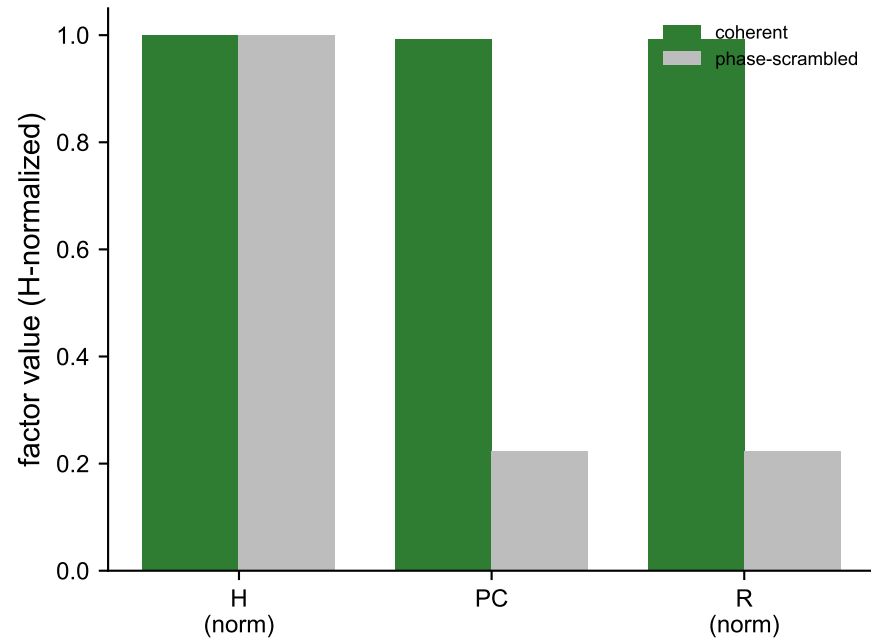
B. Phase-scramble ( |FFT| kept): H unchanged, PC & R collapse
