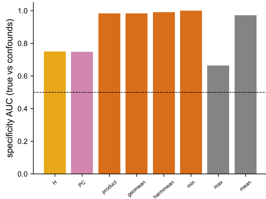
A. Independent factors: conjunctions beat both factors & disjunctions
