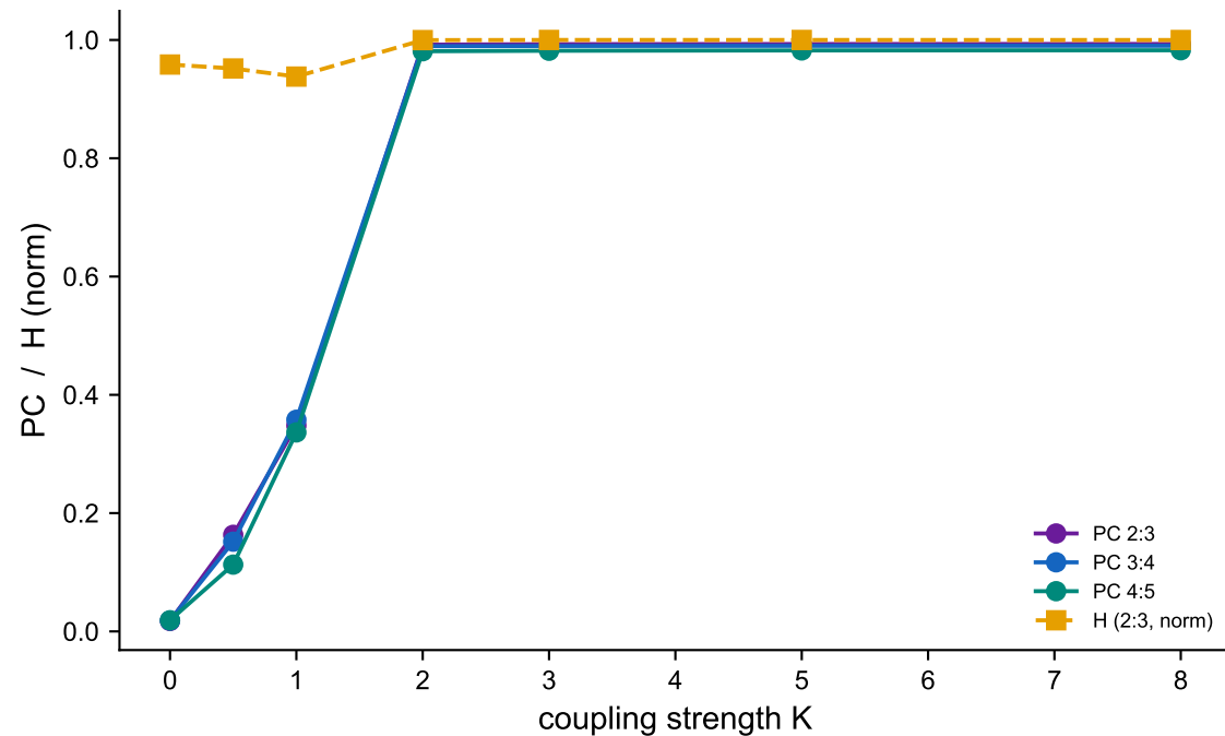
A. Polyrhythmic phase coupling rises with K (H flat: blind to coupling)
