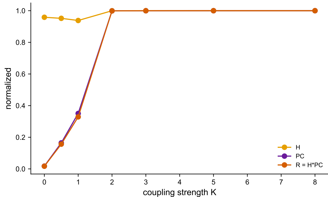
B. R tracks emergent coupling (2:3) \rho(\text{PC}, K) = +1.00 , \rho(H, K) = +0.71
