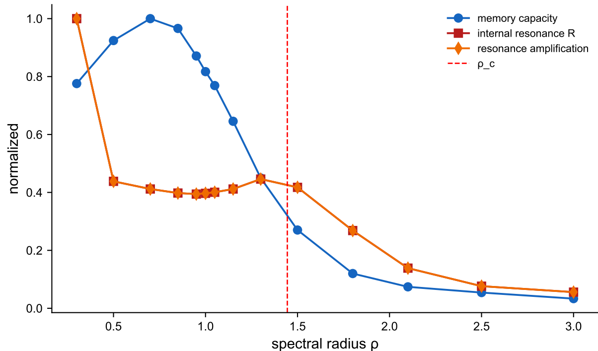
B. Resonance vs computation vs criticality MC peaks \rho=0.70 , R peaks \rho=0.30
