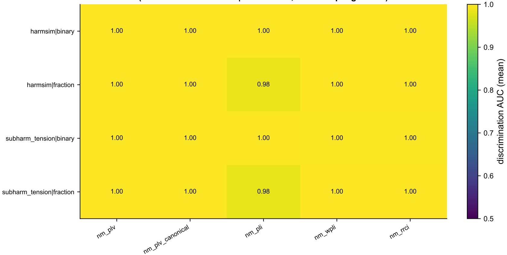
Study 4 — Strategy comparison: harmonic-signal discrimination AUC (rows: harmonic kernel | ratio kernel; cols: coupling metric)
