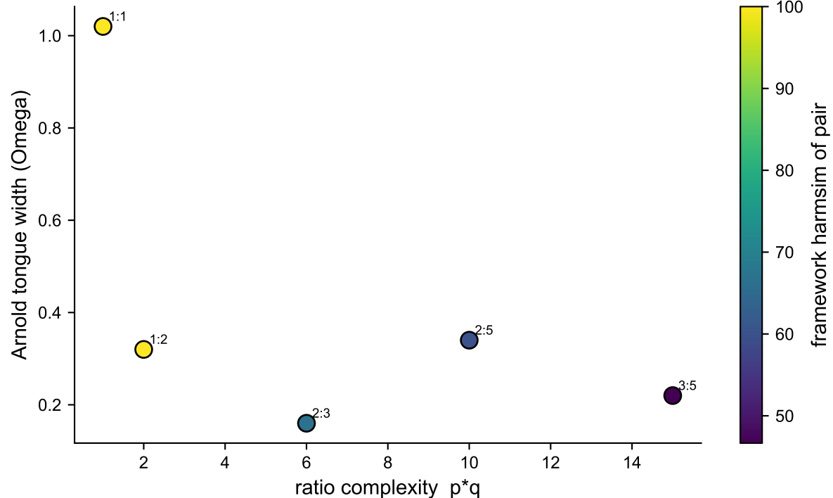
B. Lockability vs harmonic complexity \text{width} \sim \text{complexity } \rho = -0.50 , \text{width} \sim \text{harmsim } \rho = +0.41
