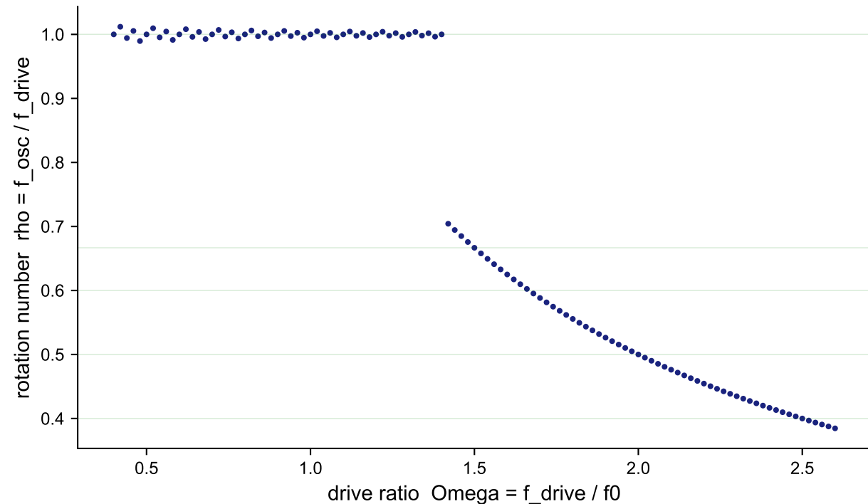
A. Devil's staircase (forced Van der Pol) plateaus = Arnold tongues; wider at simple ratios
