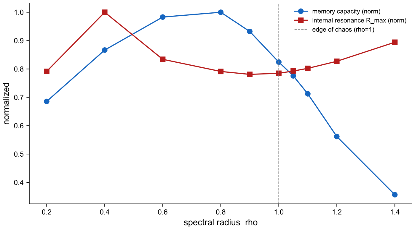
Study 9 — Reservoir: resonance vs computational regime Spearman(R, MC) = -0.32; argmax rho: MC=0.80, R=0.40
