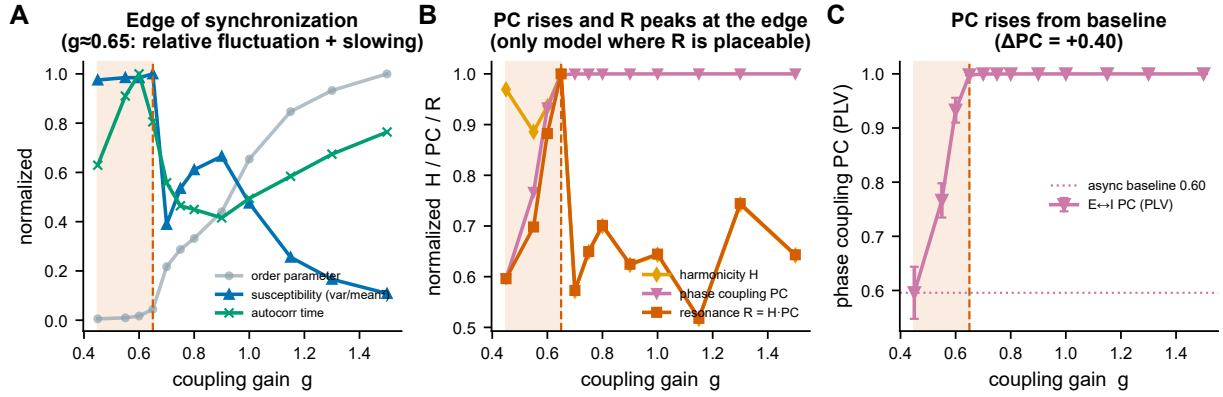
Figure 4. At the synchronization onset, phase coupling and resonance become placeable. (A) The edge of synchronization, located by the relative-fluctuation susceptibility ( \text{var}/\text{mean}^2 ) and the autocorrelation time (critical slowing), which peak together near g \approx 0.65 (shaded); raw envelope-variance susceptibility peaks later, an amplitude confound. (B) The resonance factors against the edge: harmonicity H , phase coupling PC , and R = H \cdot PC (normalized); PC rises through the edge and R peaks at it — this is the only one of the three models where R is non-trivial, because sustained oscillations and criticality coexist. (C) The absolute rise of E \leftrightarrow I phase coupling (PLV) above its non-zero asynchronous baseline ( \Delta PC = +0.40 ).
