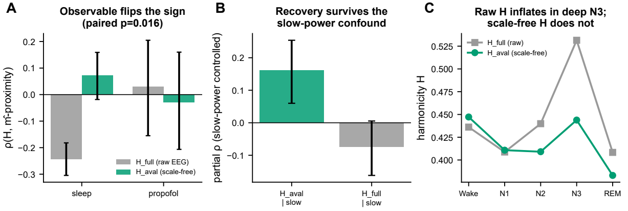
Figure 6. The reversal is an observable-choice effect. (A) On the scale-free population signal ( H_{aval} ) harmonicity tracks criticality positively , while on the raw oscillatory signal ( H_{full} ) it reverses — a paired per-subject sign dissociation. (B) The scale-free recovery survives controlling for slow-band power (partial \rho ). (C) Across sleep stages, raw H rises into N3 while the scale-free H does not, recovering the model prediction on the correct observable.
