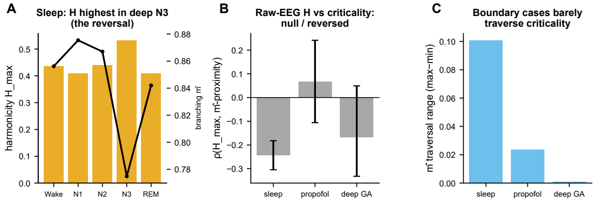
Figure 5. In human EEG the prediction reverses. (A) In sleep, raw-EEG harmonicity H_{\max} is highest in deep N3 — the most subcritical state (branching \hat{m} overlaid). (B) Per-subject Spearman \rho between H_{\max} and criticality proximity is null or negative across datasets. (C) Boundary cases: propofol sedation and deep anaesthesia barely traverse criticality (small \hat{m} range), so they cannot test the law; the real-data test rests on the sleep traversal.
