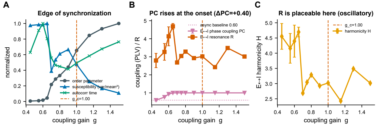
Figure 4. At the synchronization onset, phase coupling becomes a marker. (A) Order parameter, normalized susceptibility ( \text{var}/\text{mean}^2 ) and autocorrelation time locate the synchronization onset g_c . (B) E \leftrightarrow I phase coupling rises above its non-zero asynchronous baseline at the onset ( \Delta PC ); resonance R becomes non-trivial. (C) Harmonicity across g : this is the one model where R is placeable, because oscillations and criticality coexist.
